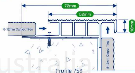
PROFILE TYPICAL INSTALLATION Screw Fixed
